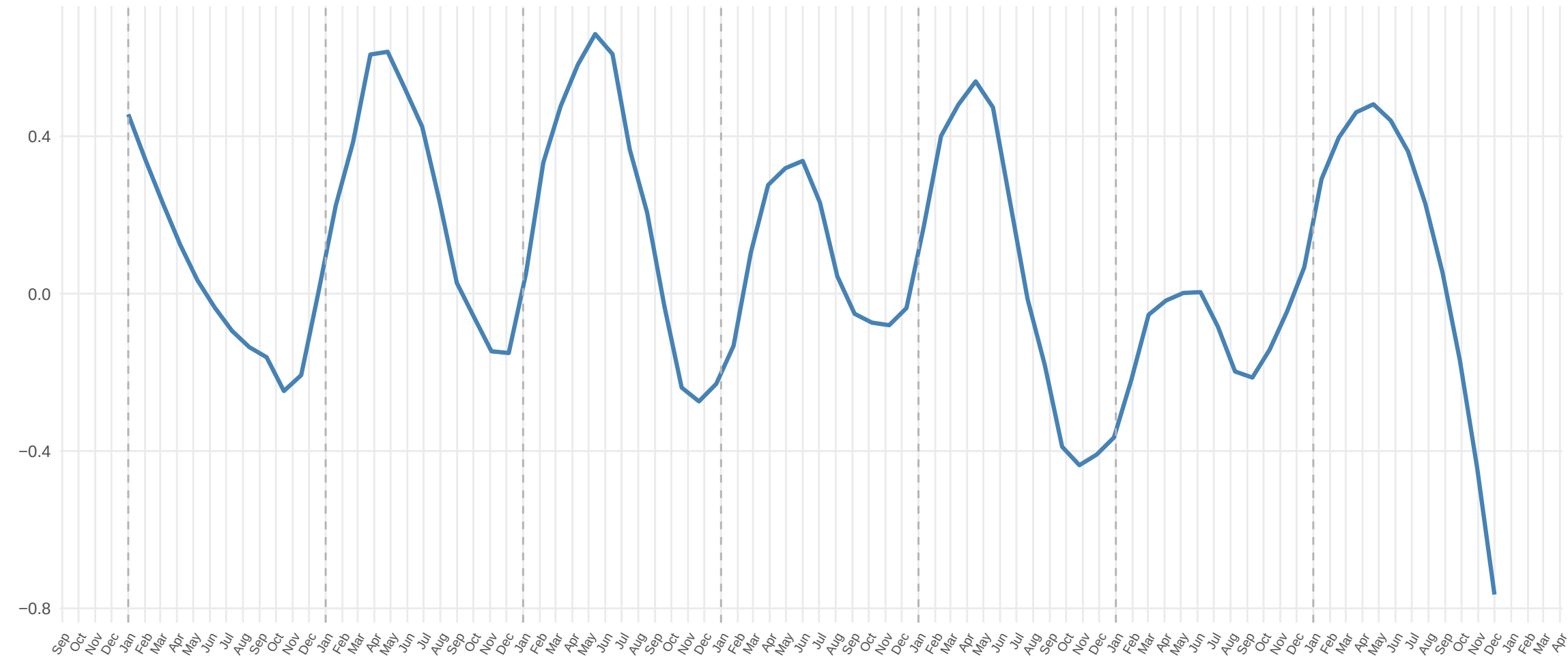
wind
