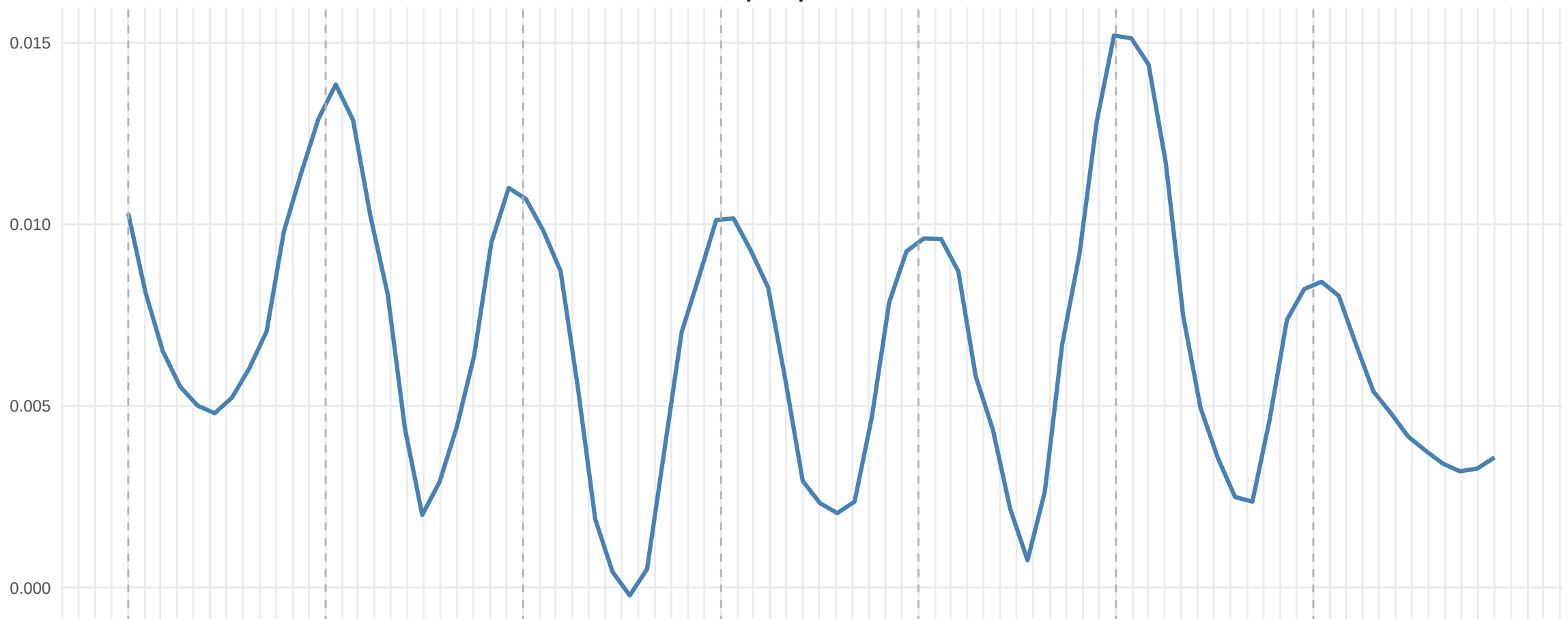
precipitation
