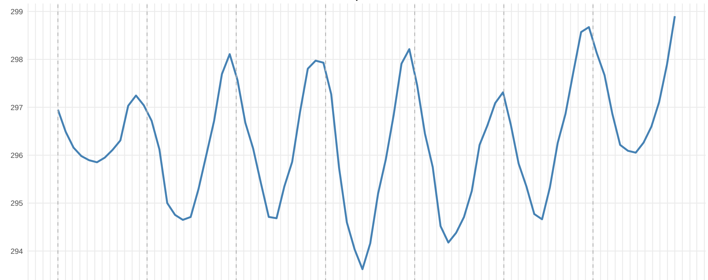
temperature
