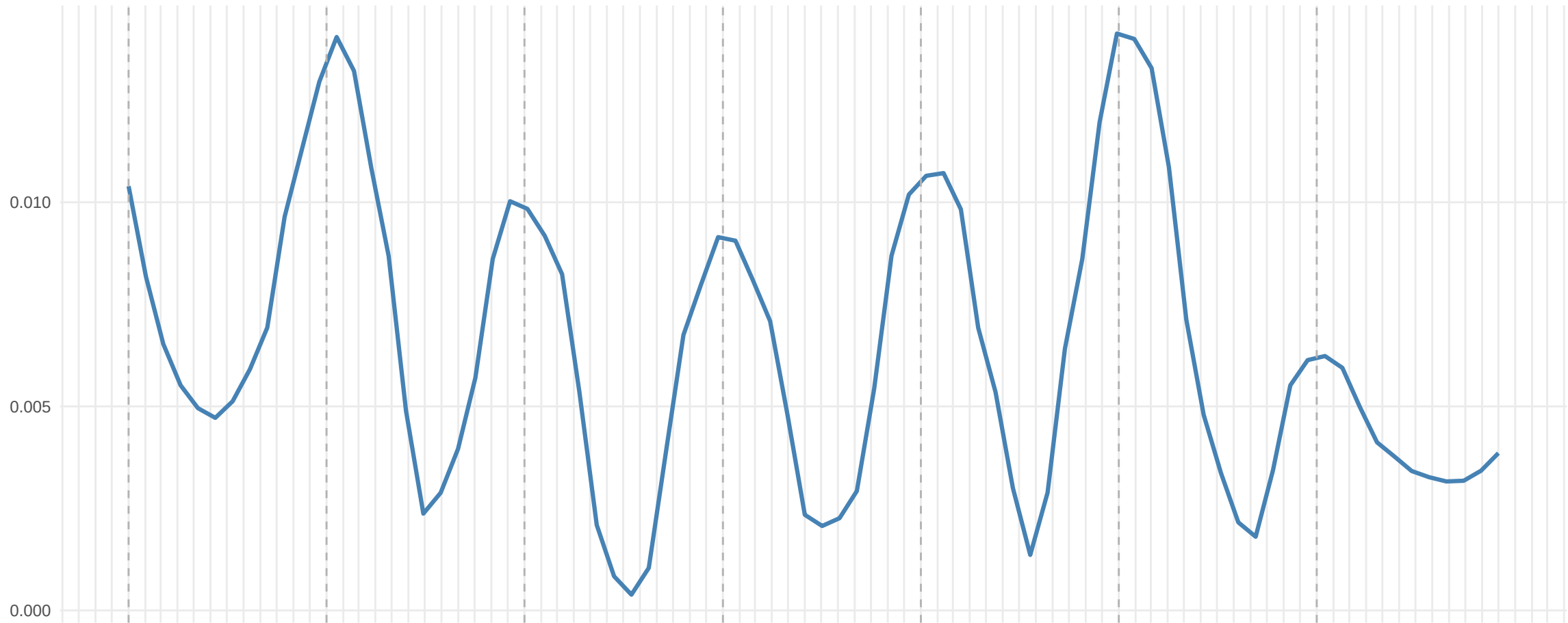
precipitation
