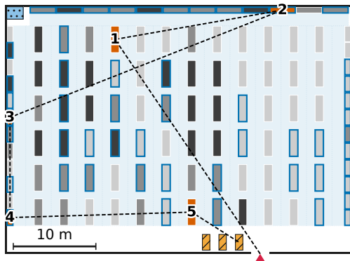
As built (repaired): tour 128 m
