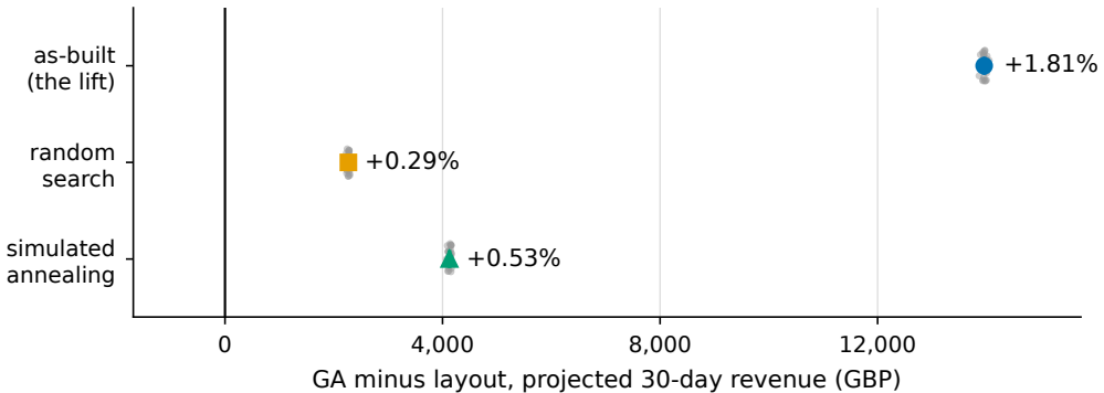
UCI store, paired over 30 held-out MC re-evaluations (95% intervals)
