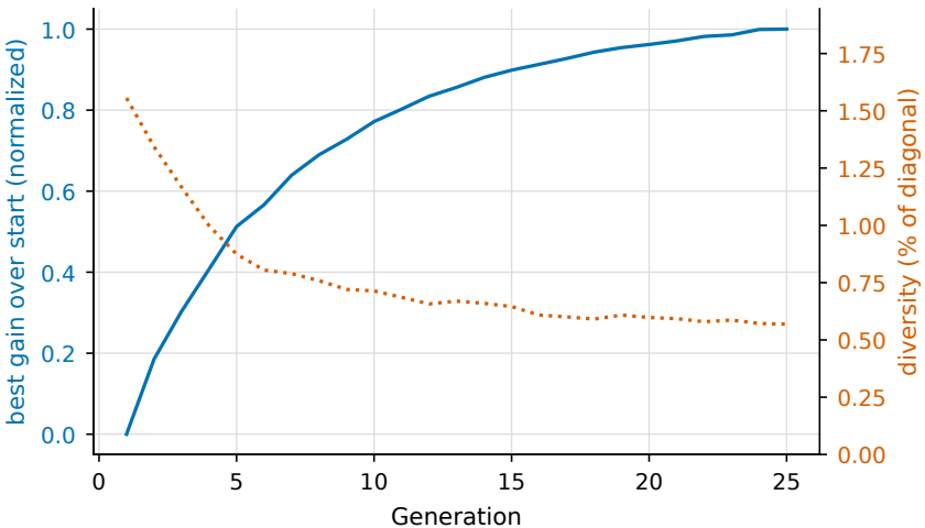
Mutation 0.18, population 30; 30 runs
