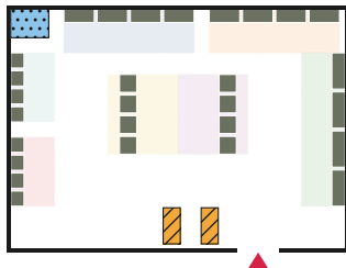
Electronics (racetrack), 32×22 m 10 sections, 80 items, 3 lanes
