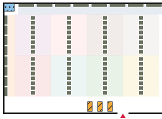
Clothing (freeform), 32×22 m 10 sections, 80 items, 3 lanes
