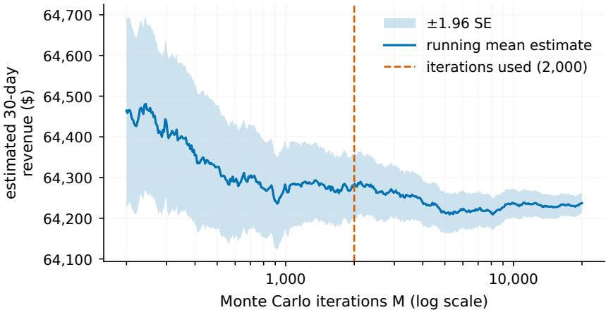
Monte Carlo estimator convergence, SE \propto 1/\sqrt{M}
