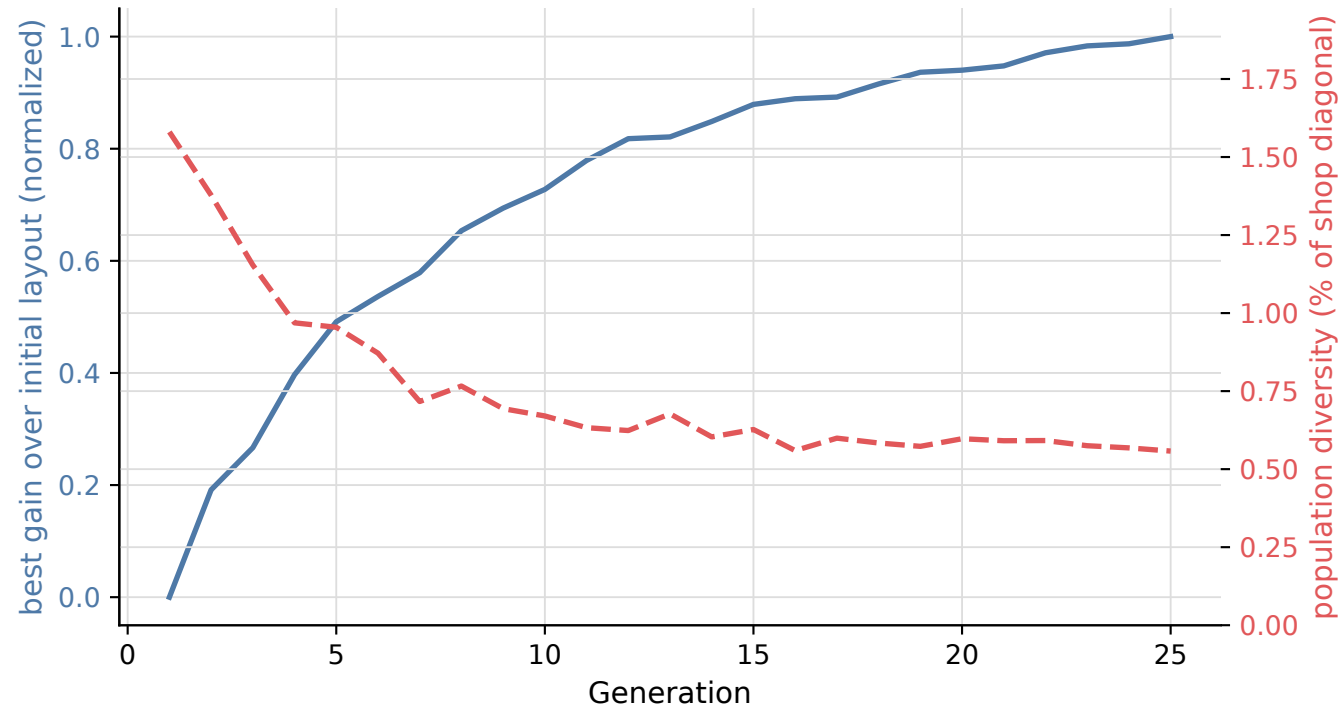
GA convergence vs population diversity (default 0.18, pop 30; 6 runs)
