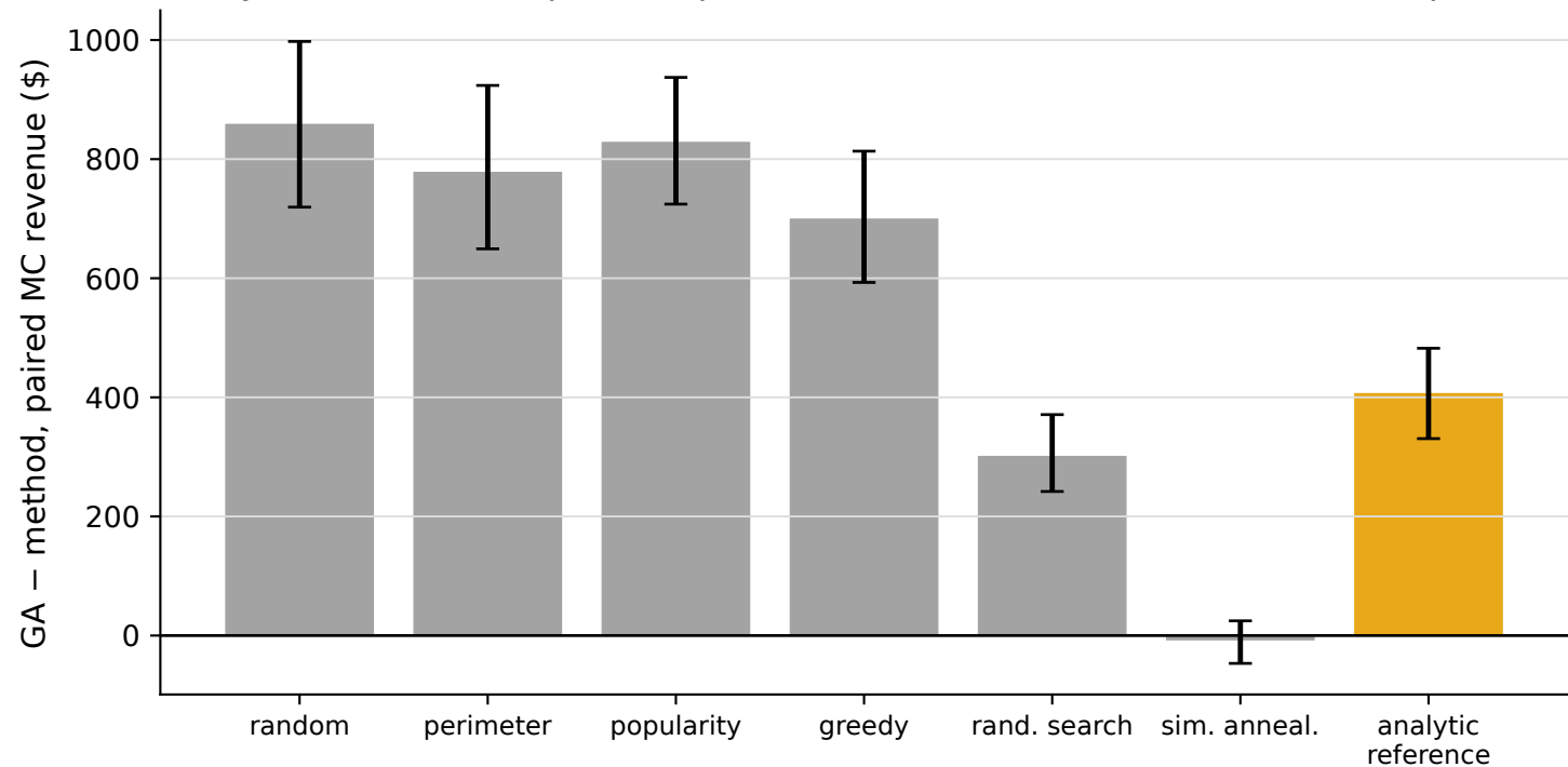
Layout method comparison: paired differences (99.3% cluster-bootstrap CIs)
