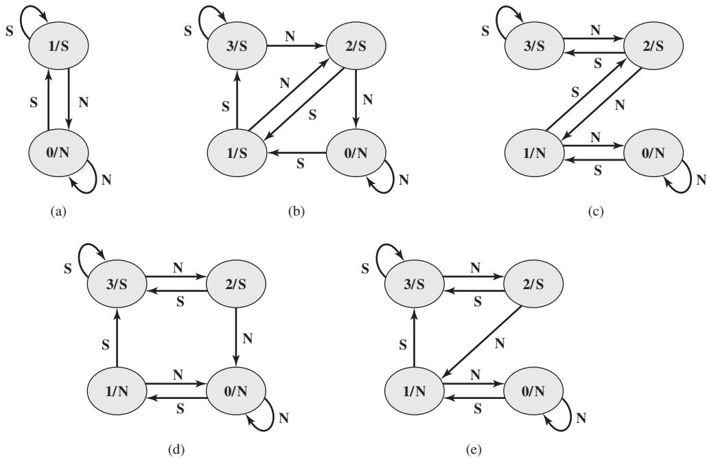
Figura 14.17. Figura del Problema 14.8. S = hay salto ( branch taker ); N = no hay salto ( branch not taken ).
