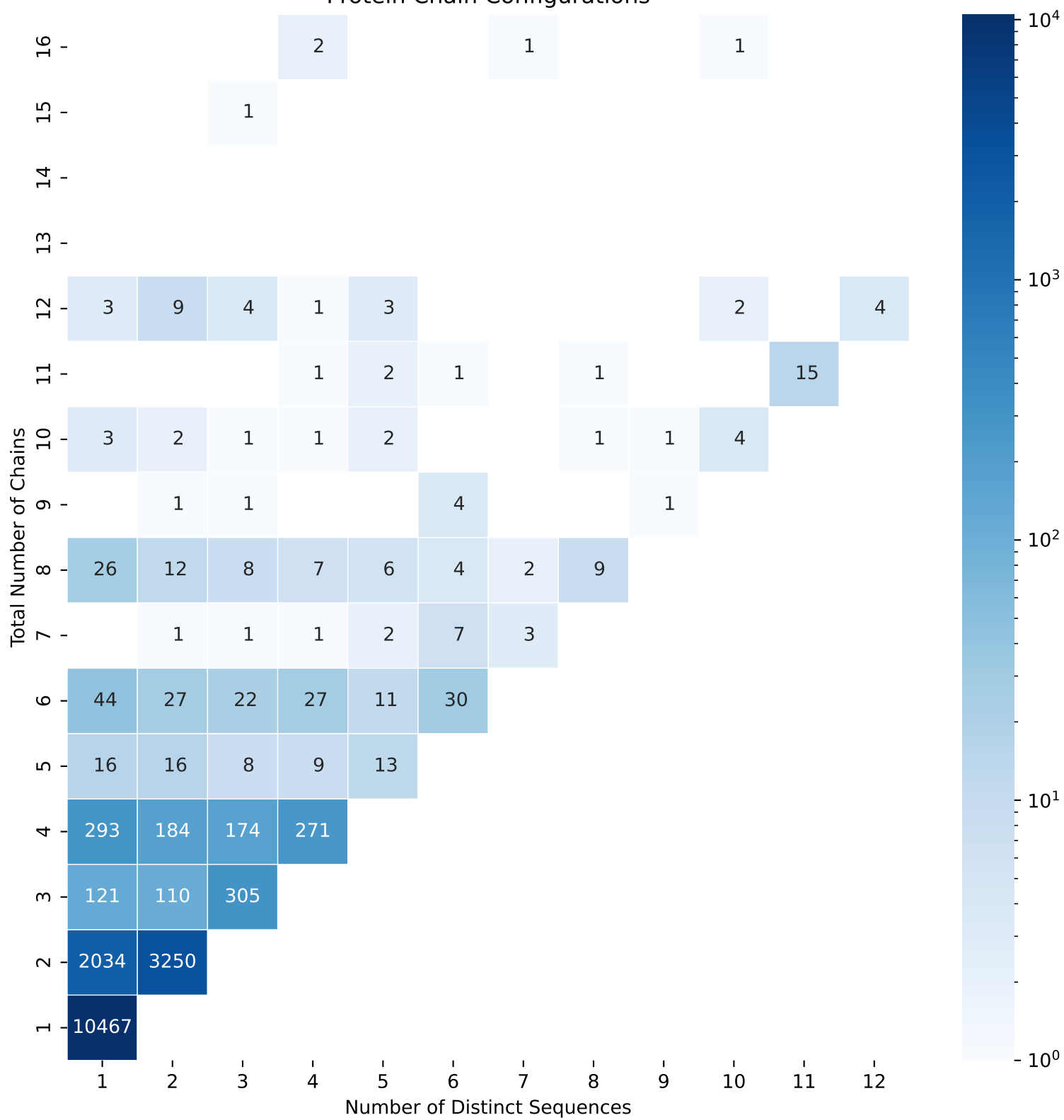
Protein Chain Configurations
