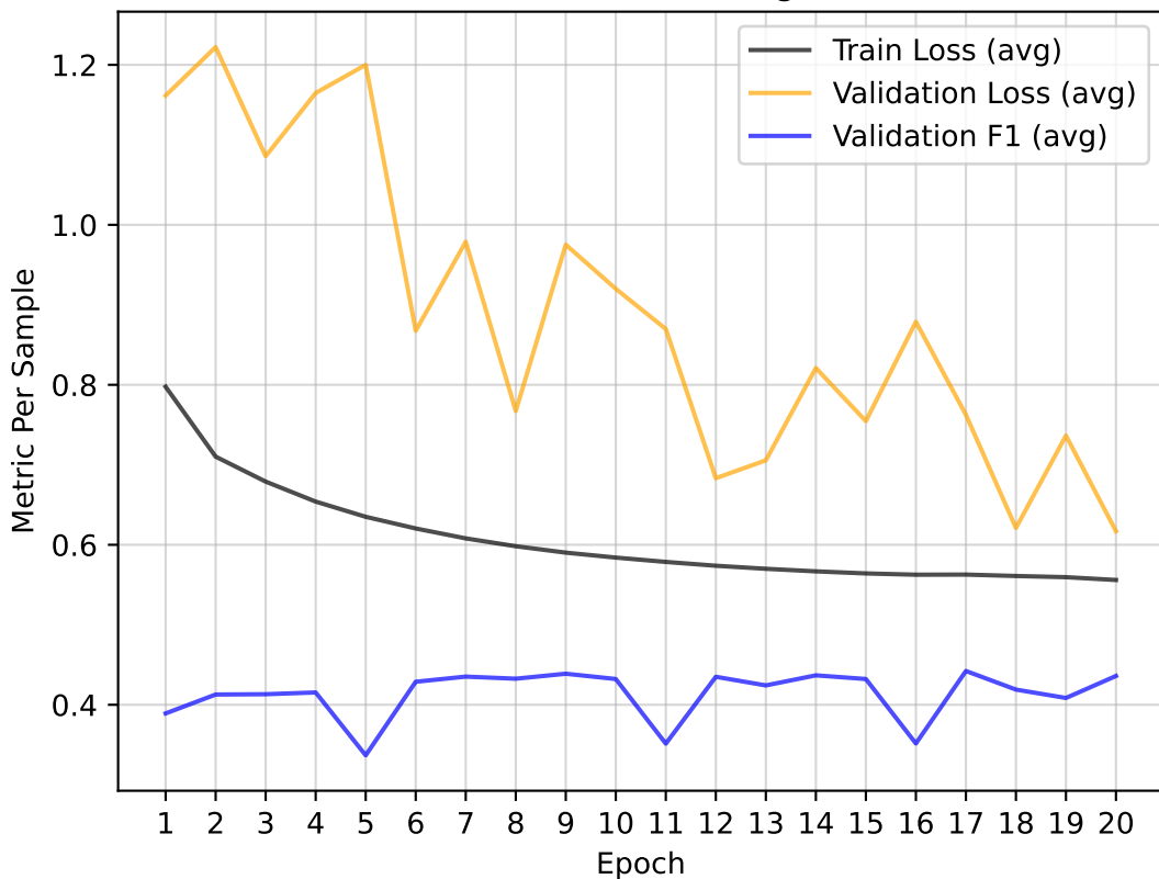
Cross Validation Learning Curves
