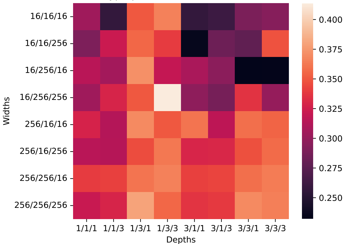
Broad Hyperparameters Search, attribute: f1
