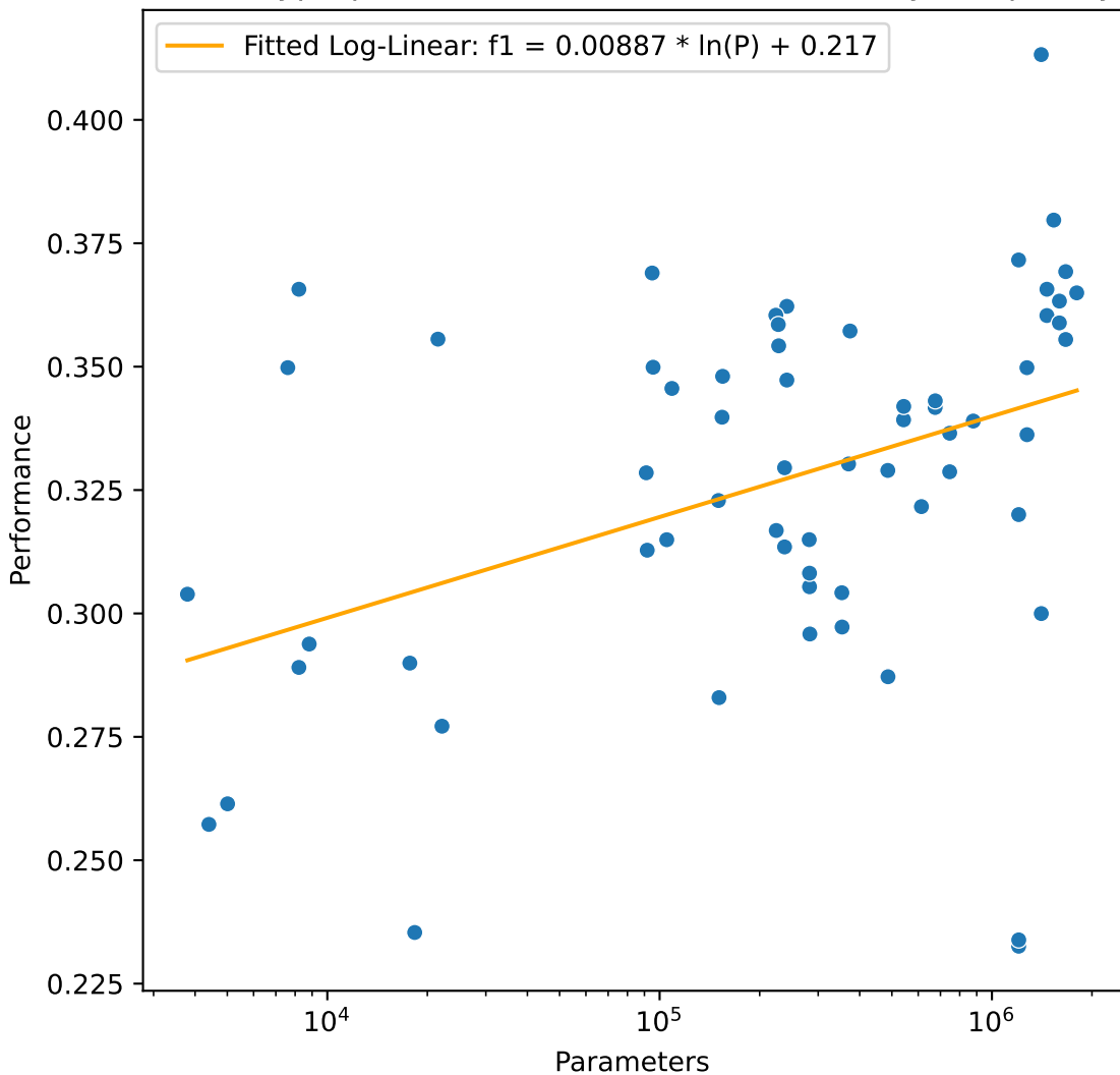
Broad Hyperparameters Search, attribute: f1 by complexity
