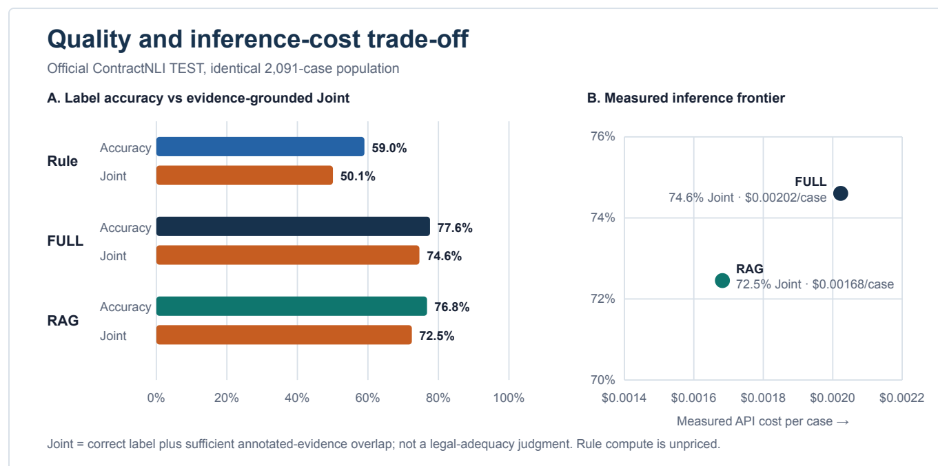
Figure 4. Architecture quality versus cost (official TEST, n=2,091 ).
