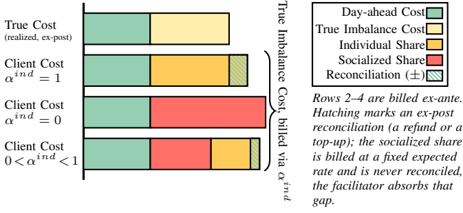
Fig. 4: A consumer's billed cost across individualization grades \alpha^{ind} (schematic; not to scale). Top: realized ex-post cost. Below: ex-ante billed cost under full individualization, full socialization, and a mixed case. Only the individualized share is reconciled (hatched, Eq. 21); the socialized share is billed at a fixed expected rate and never reconciled, so the facilitator absorbs its ex-post deviation.
