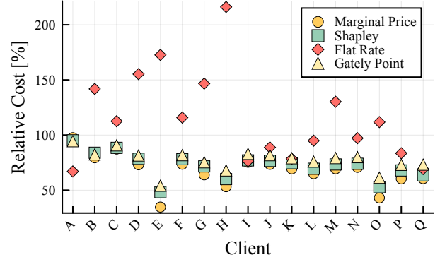
Fig. 6: Plot of ratio between allocated cost and singleton cost
