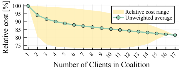
Fig. 5: Plot of ratio between cost as part of the grand coalition and as part of a subcoalition, shaded area showing the range of relative costs for coalition size. Remove legend, explain here
