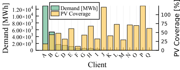
Fig. 3: Bar chart of total PV coverage and demand of consumers in the case study period
