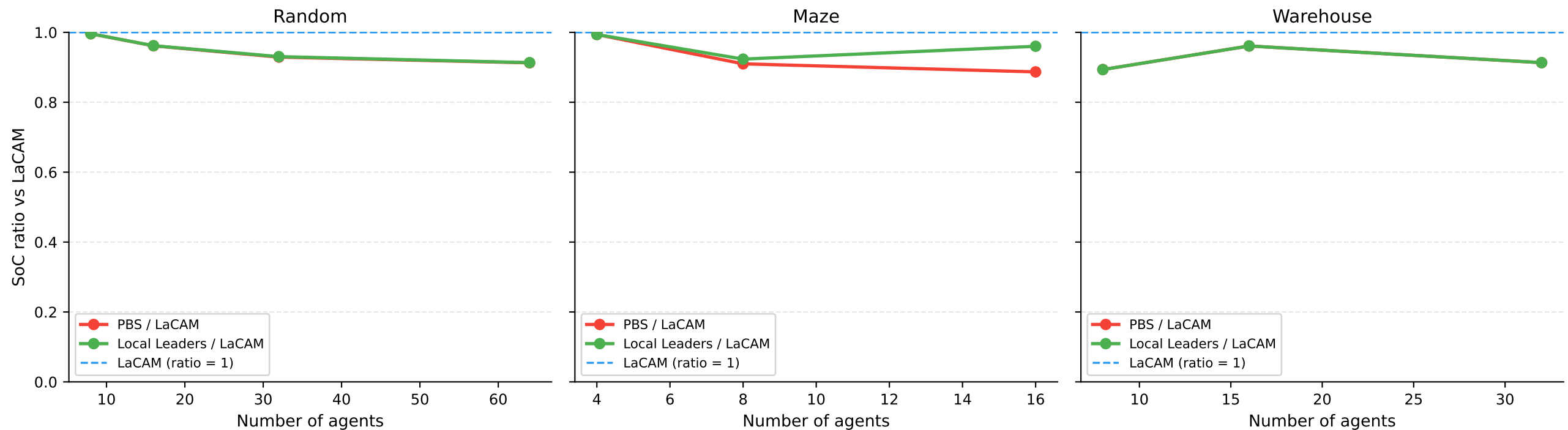
SoC Ratio vs LaCAM (< 1 = better than LaCAM)
