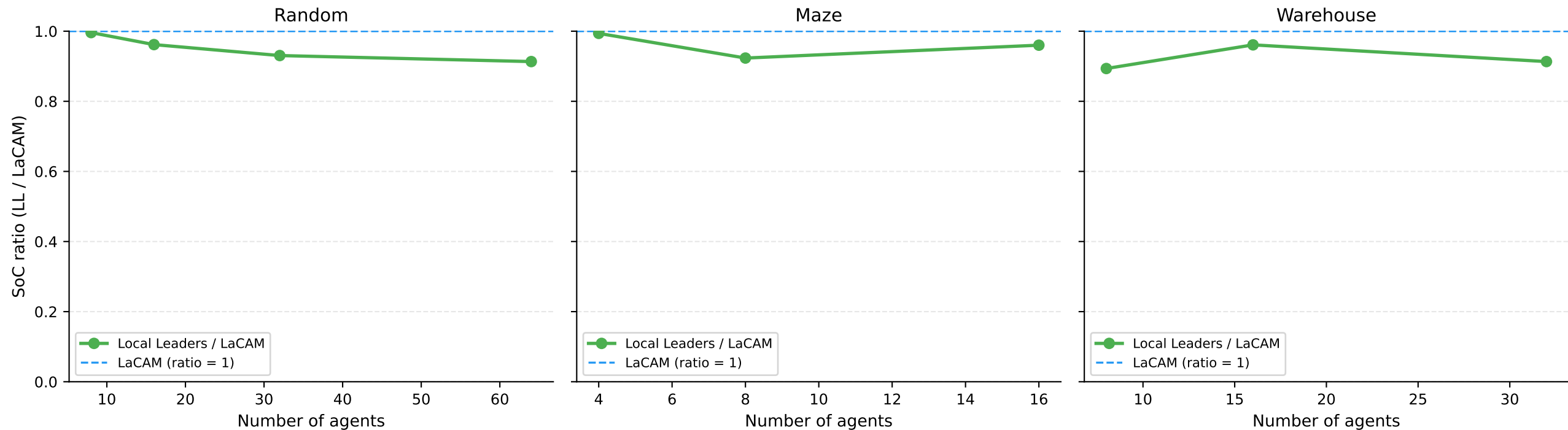
SoC Overhead: Local Leaders vs LaCAM (ratio > 1 = worse than LaCAM)
