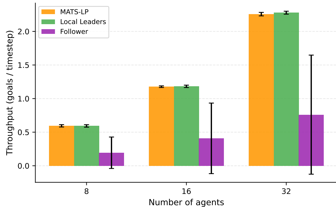
Random maps, 0% obstacles
