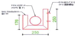
DETAIL DUDUKAN PIPA @2.5M 管道支座详图@2.5M SKALA 1:500
