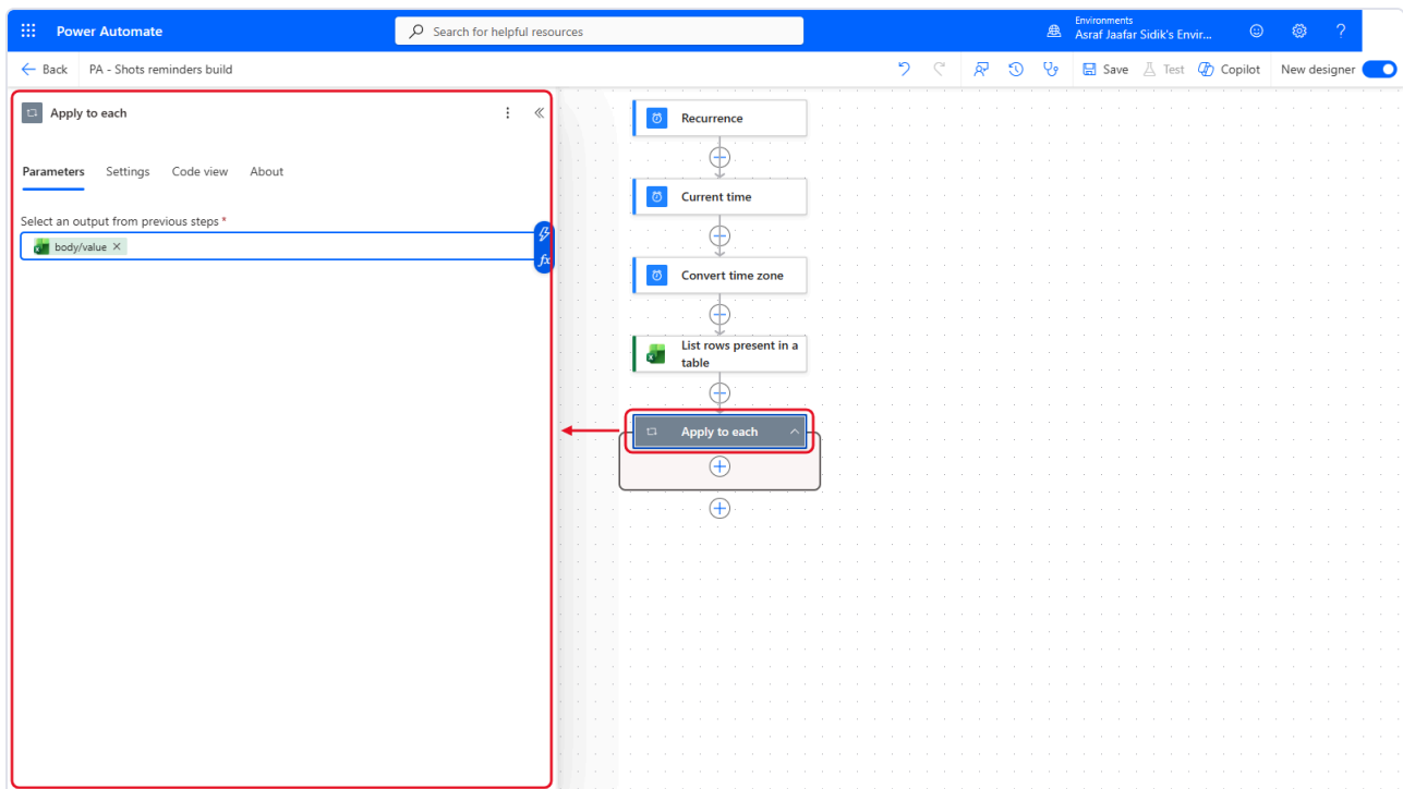
An empty Apply to each at the bottom.
