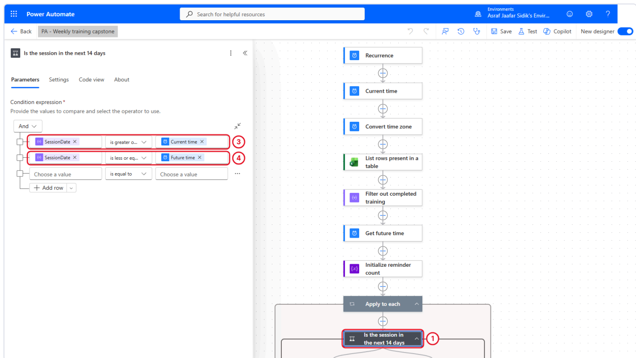
Two rules joined by AND: on or after now, and on or before 14 days from now.
