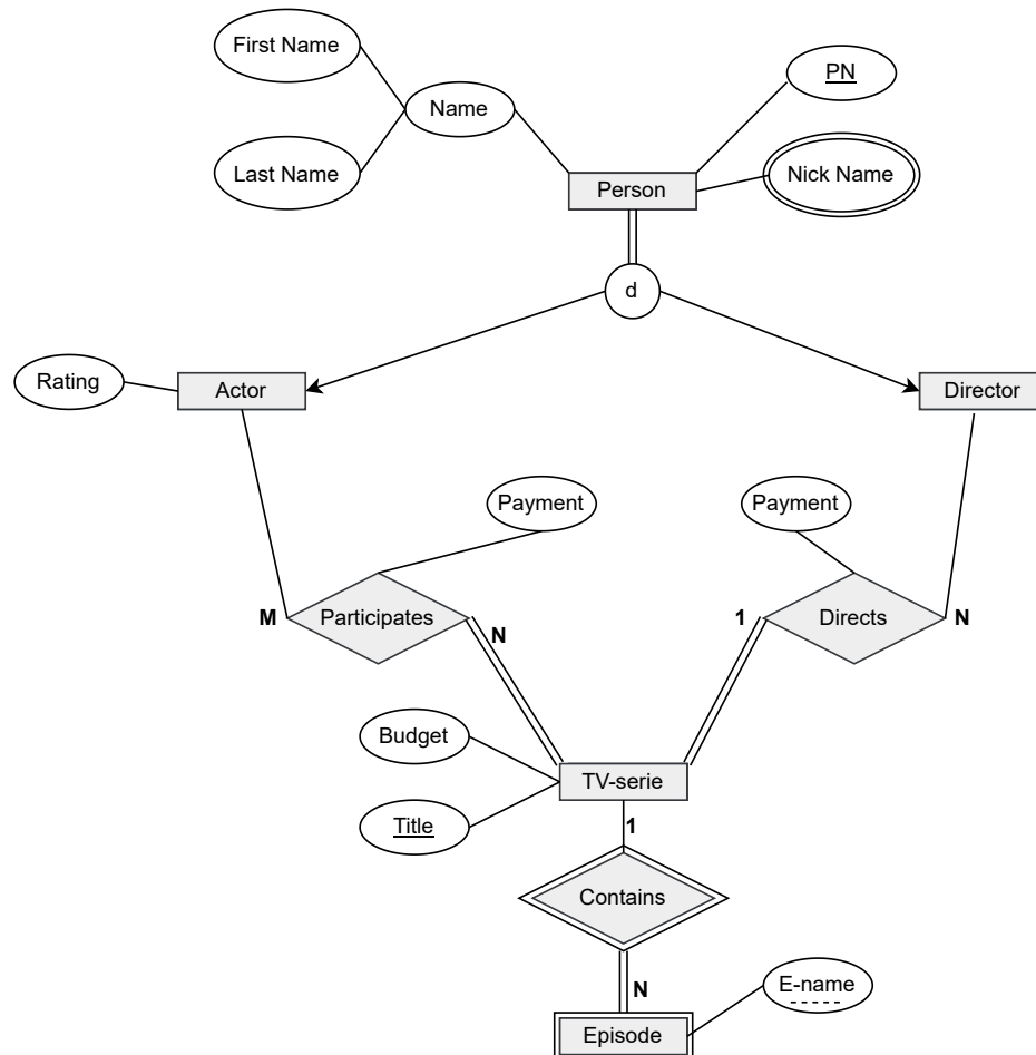
Figure 1: EER diagram that describes the relation between entities in Task 1.
