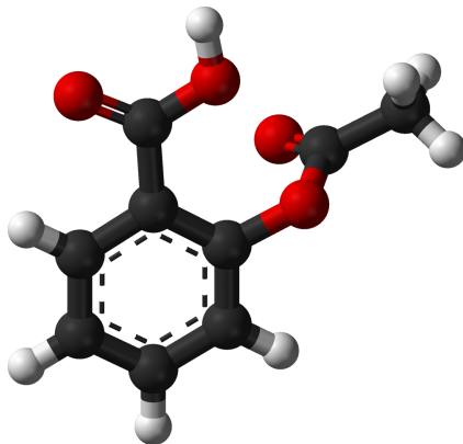
Figure 1: Ball and stick diagram of C_9H_8O_4 (Aspirin).
