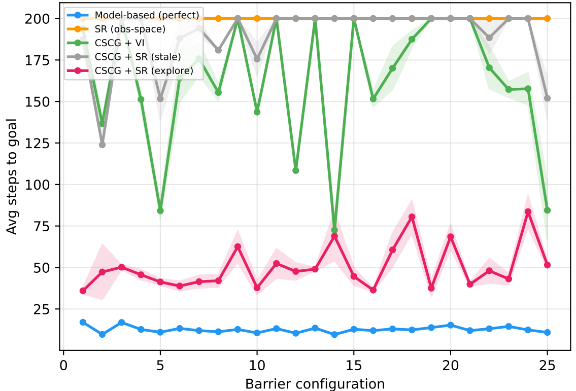
cothi-10x10 — By barrier config
