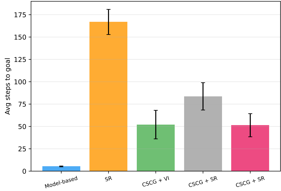
cothi-10x10 — Open arena
