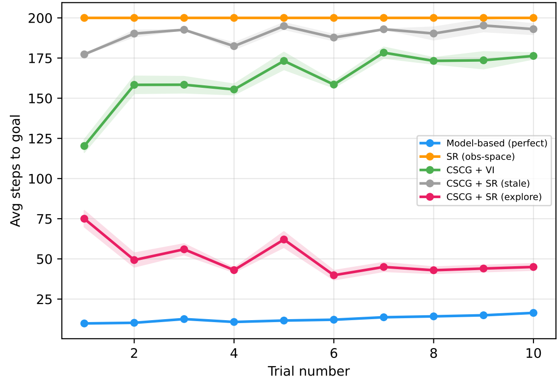
cothi-10x10 — Across trials (Cothi-style)
