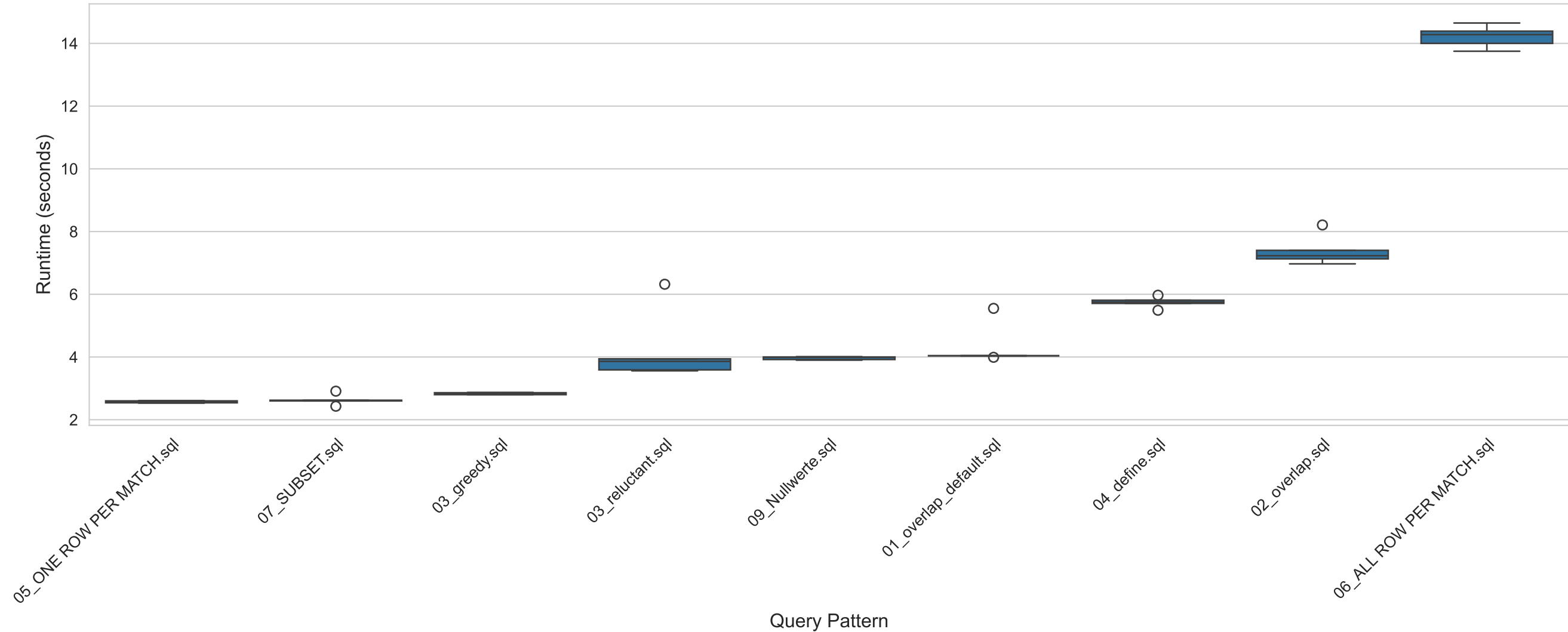
Runtime Comparison Across Query Patterns (Median + Quartiles)
