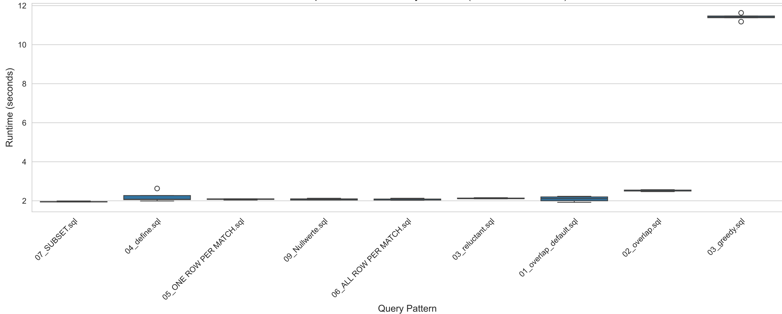
Runtime Comparison Across Query Patterns (Median + Quartiles)
