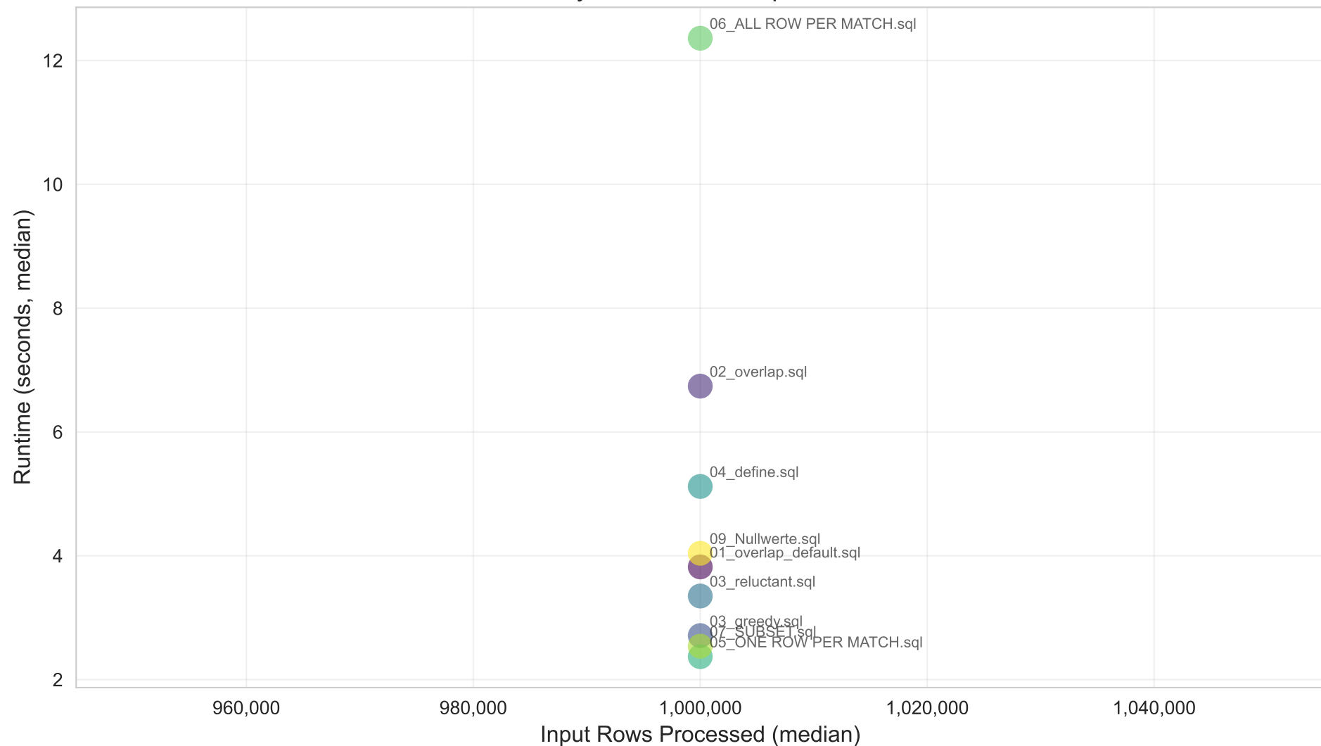
Scalability: Runtime vs. Input Data Size
