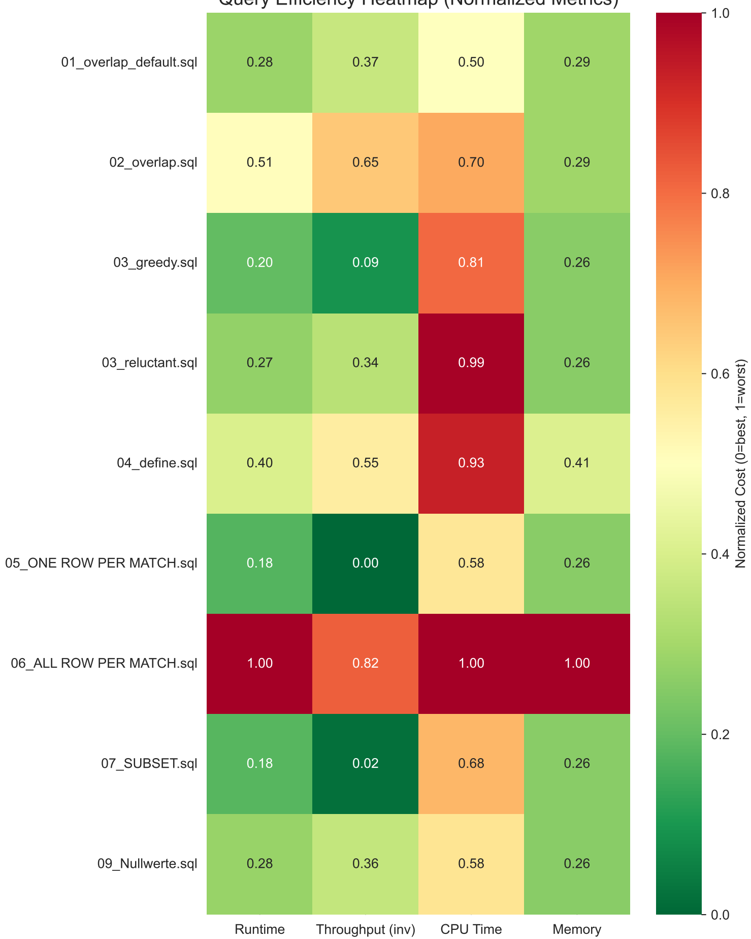
Query Efficiency Heatmap (Normalized Metrics)
