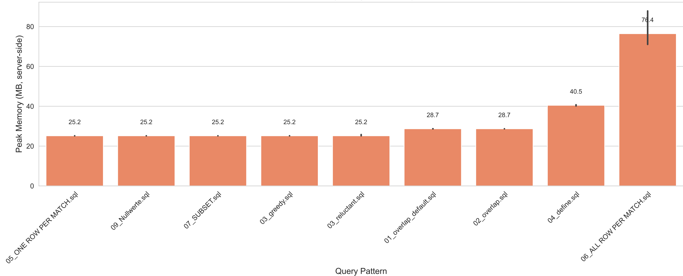
Server Memory Usage per Query Pattern
