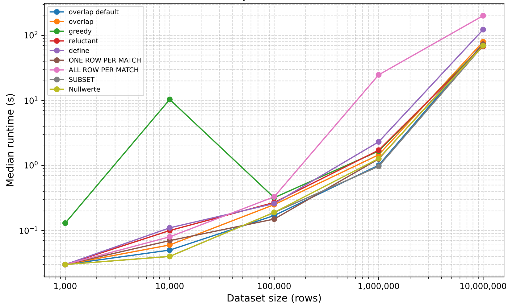
Oracle Scalability: Runtime vs. Dataset Size
