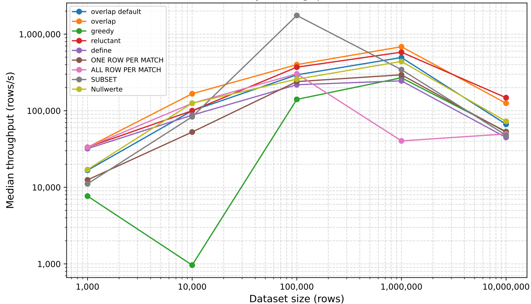
Oracle Scalability: Throughput vs. Dataset Size
