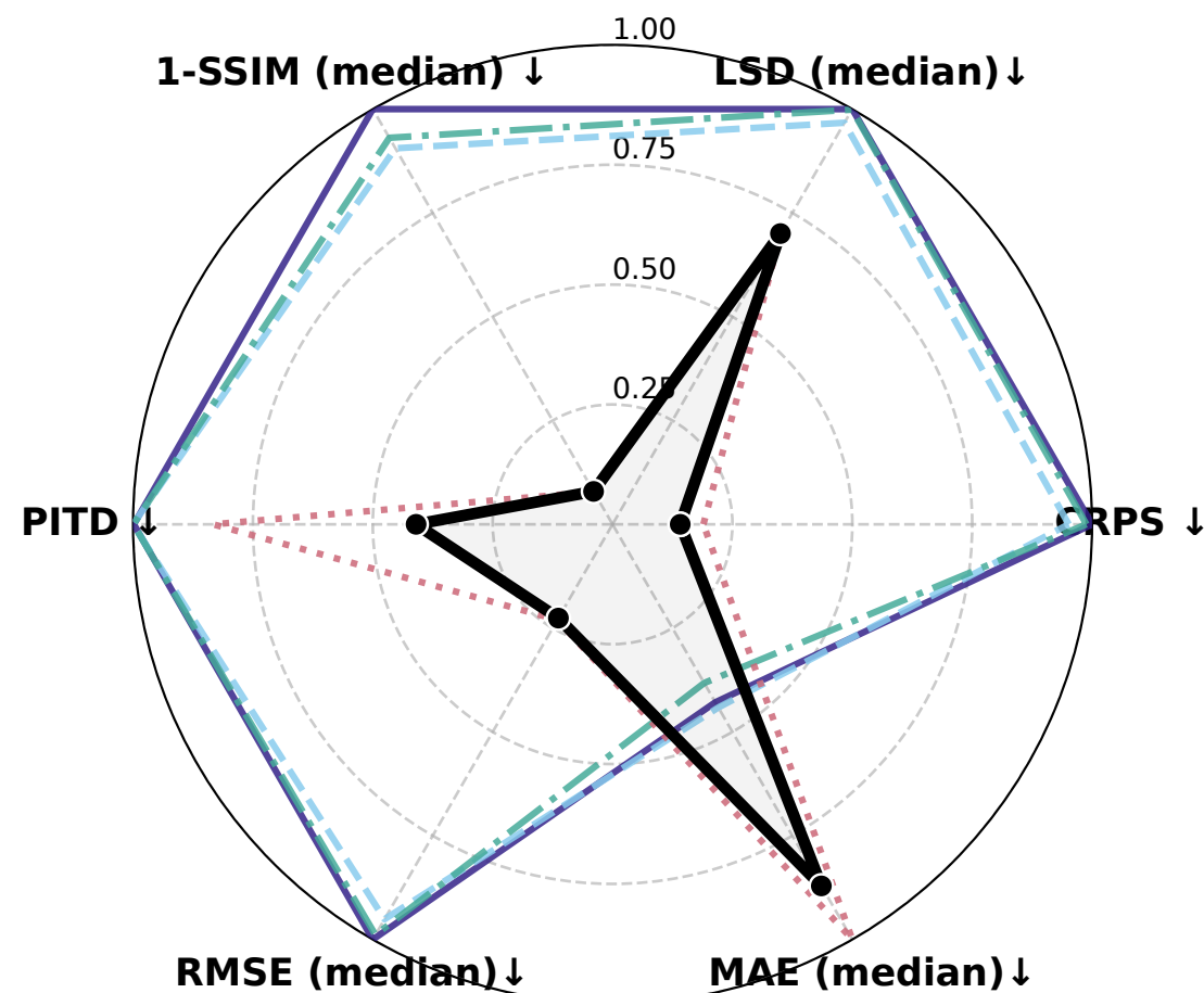
Temperature
