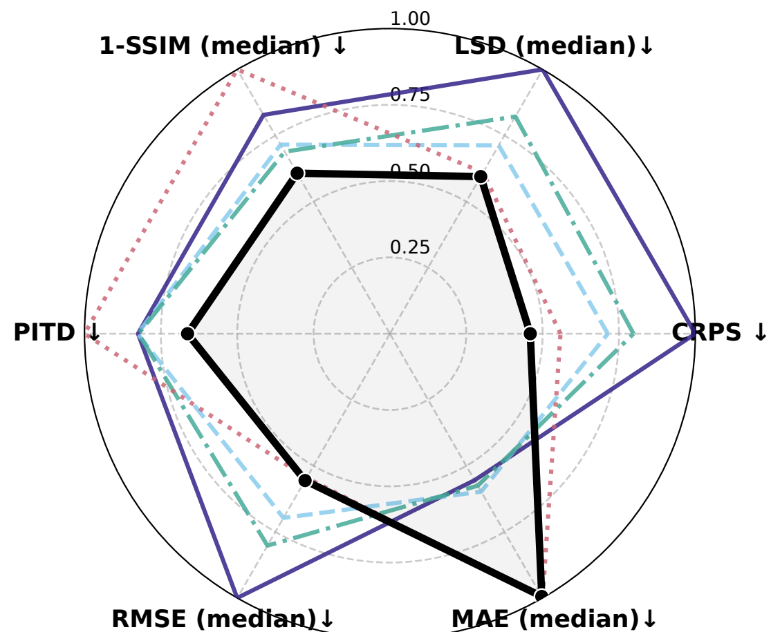
Precipitation
