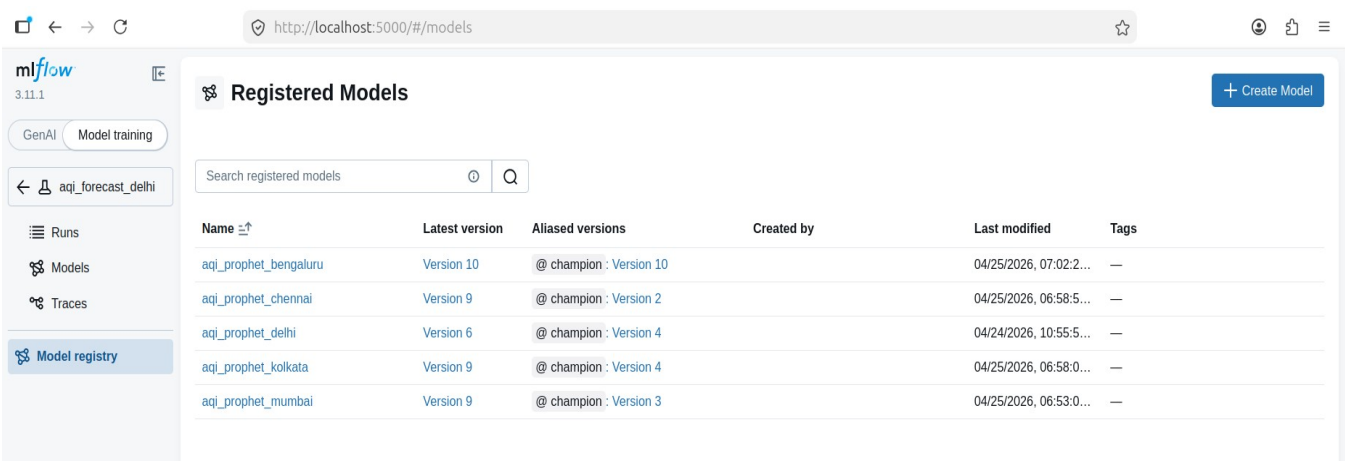
Figure 7: MLflow Model Registry — @champion alias, version history
