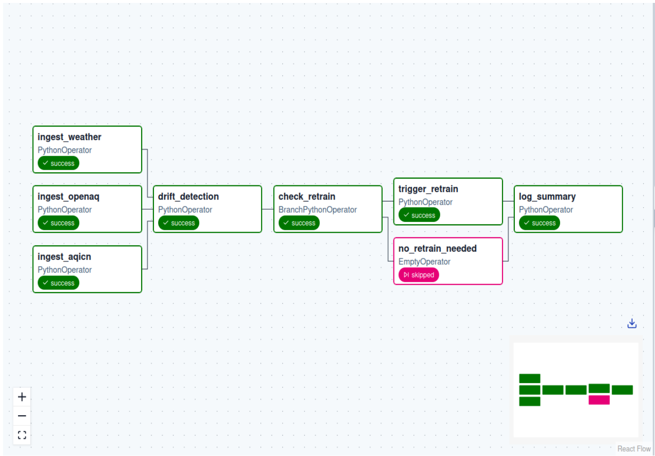
Figure 8: aqi_hourly_ingest DAG — graph view showing parallel ingest tasks
