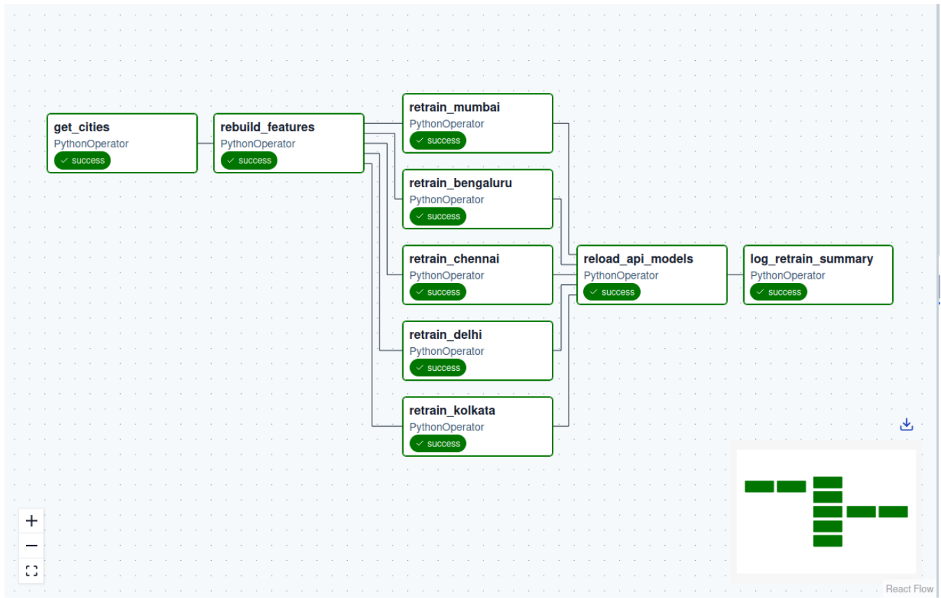
Figure 9: aqi_retrain DAG — parallel city retraining tasks
