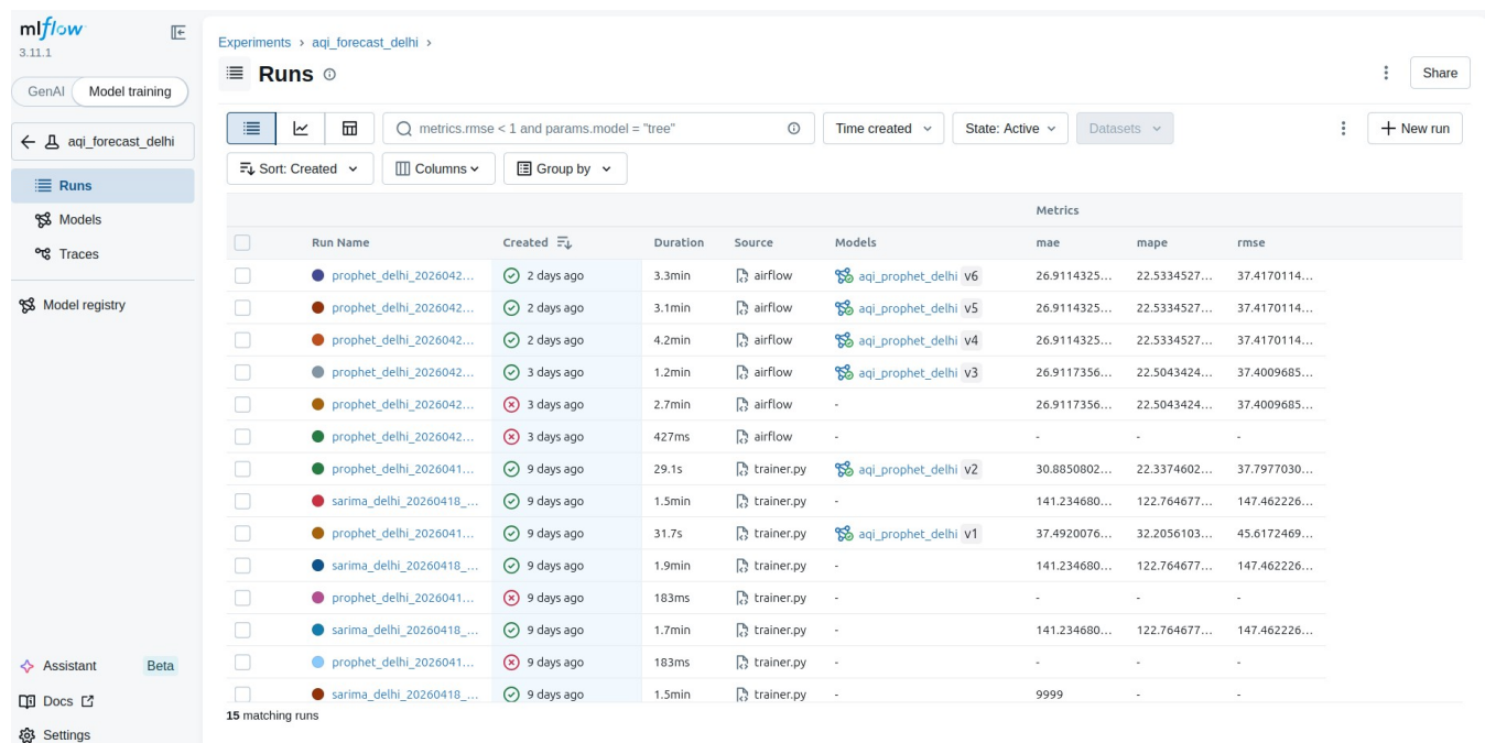
Figure 6: MLflow Experiments — runs with MAE, RMSE, MAPE metrics
