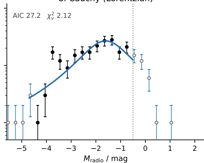
8. Cauchy (Lorentzian)
