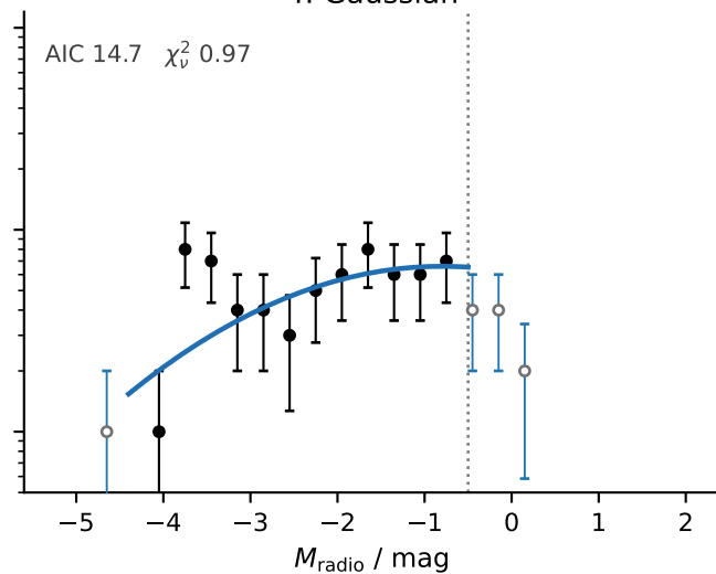
4. Gaussian
