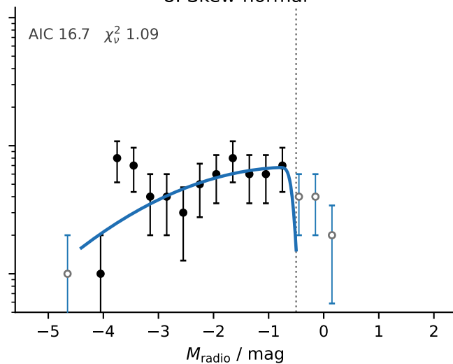
8. Skew-normal
