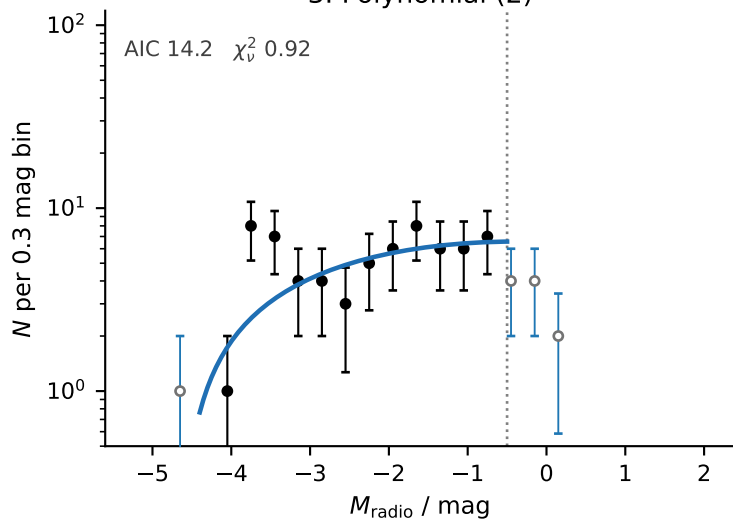
3. Polynomial (2)
