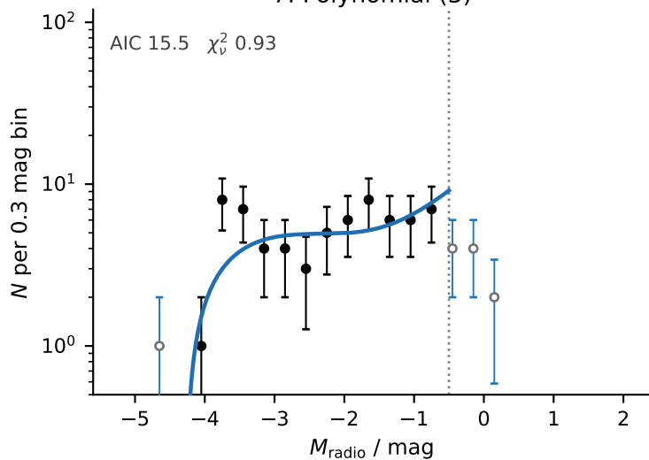
7. Polynomial (3)
