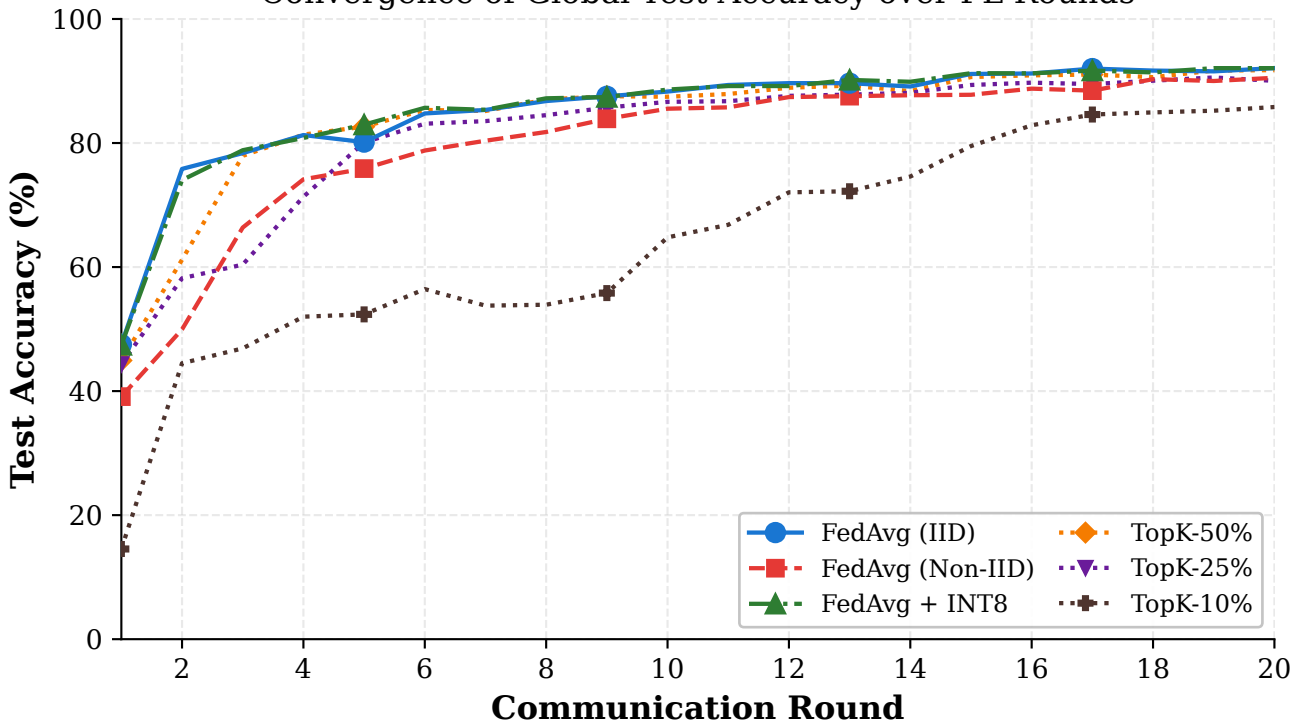
Convergence of Global Test Accuracy over FL Rounds
