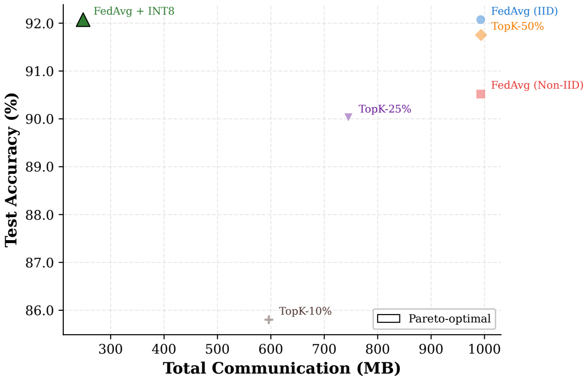
Accuracy-Communication Pareto Frontier
