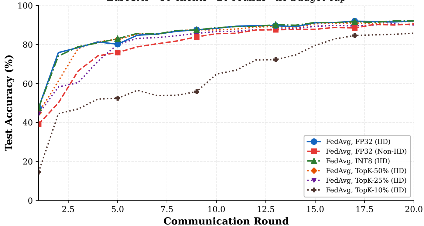
Convergence: Unrestricted FL Methods (Group A) EuroSAT · 10 clients · 20 rounds · no budget cap
