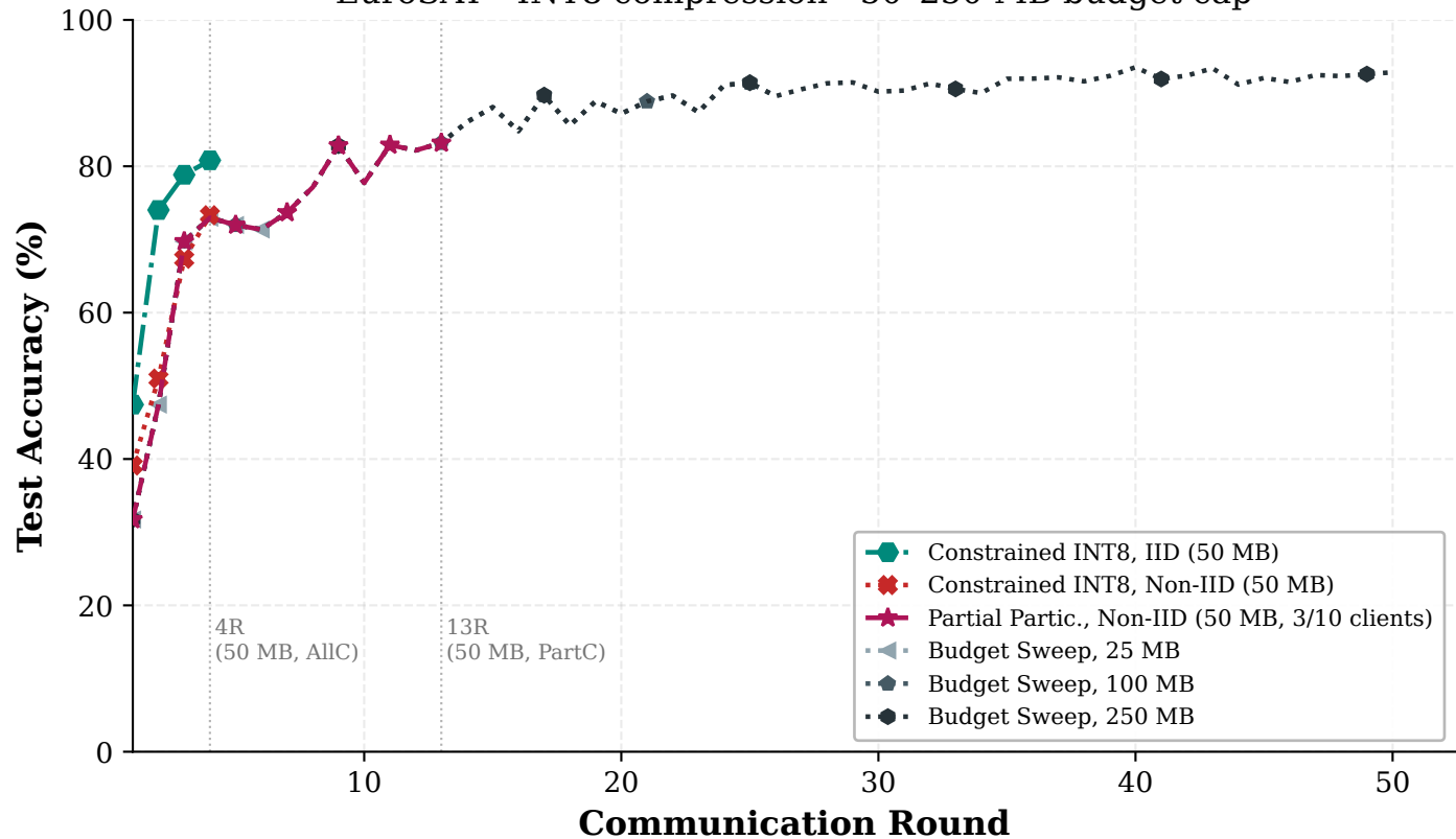
Convergence: Budget-Constrained Scenarios (Groups B & C) EuroSAT · INT8 compression · 50-250 MB budget cap
