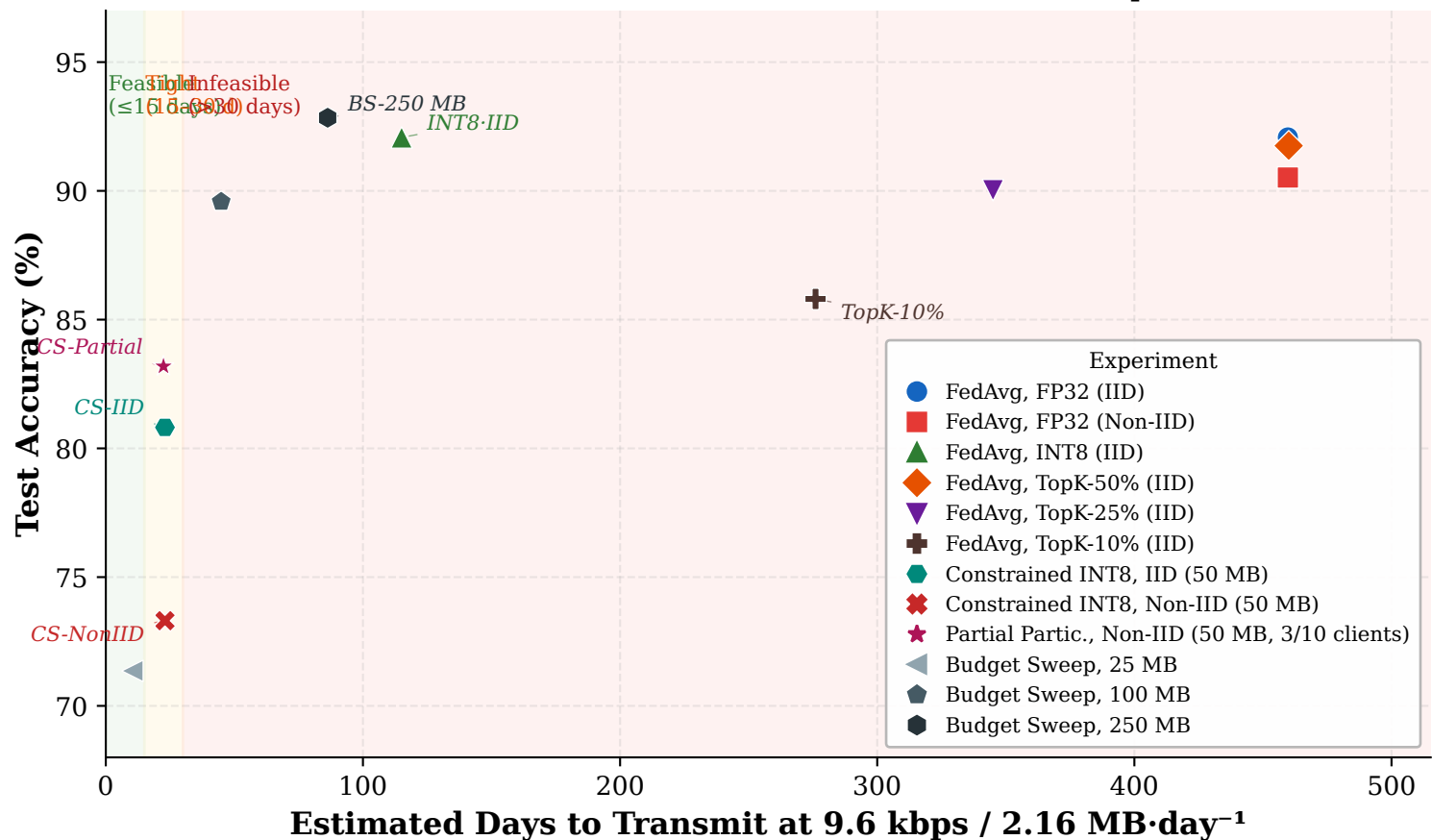
Accuracy vs. Downlink Time Requirement EuroSAT · BaselineCNN · UHF link model (9.6 kbps)
