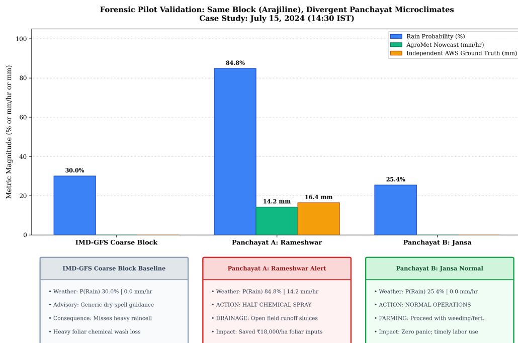
Figure 8.1: Varanasi Pilot Case Study: Divergent Panchayat Nowcasting in Rameshwar vs. Jansa under Identical Coarse Block Forecasts (July 15, 2024, 14:30 IST).
