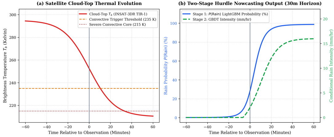
Figure 5.1: Two-Stage Hurdle Nowcasting Model: Satellite TIR Cloud-Top Depression Dynamics and Resulting Rain Probability and Conditional Intensity.
