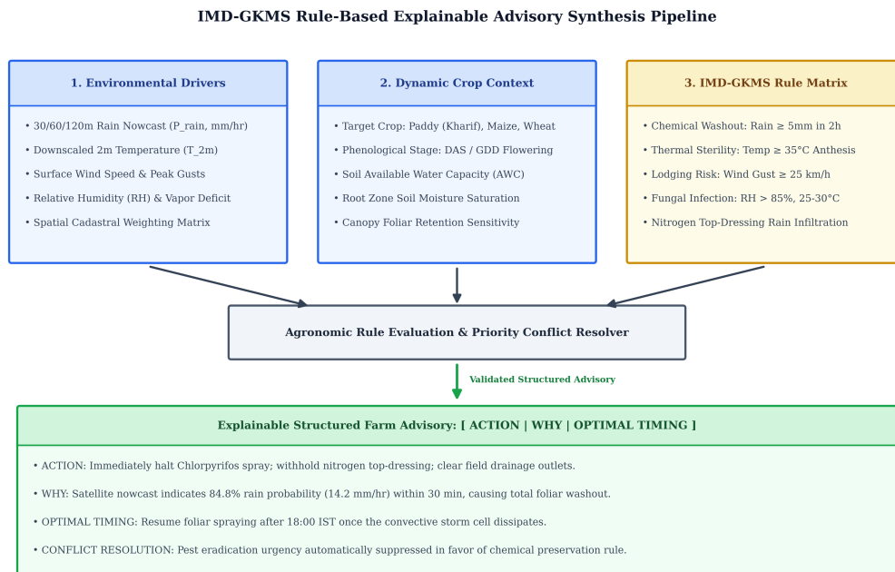
Figure 6.1: IMD-GKMS Rule-Based Explainable Advisory Synthesis Pipeline: Multi-Hazard Evaluation and Structured Action Directives.
