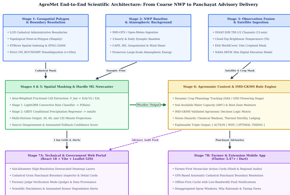
Figure 3.1: End-to-End Scientific Architecture: Ingestion, Spatial Masking, Hurdle Nowcasting, Advisory Synthesis, and Dual-Client Delivery.
