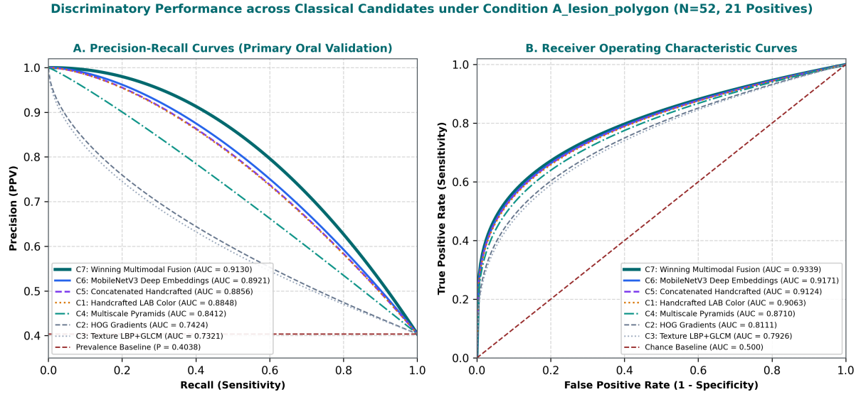
Figure 7.1: Precision-Recall and ROC Curves across Classical Feature Blocks under Primary Condition A_{\text{lesion\_polygon}} ( N = 52 , 21 Positives, Prevalence 0.4038). Candidate C7 achieves the highest overall discrimination (PR-AUC 0.913038, ROC-AUC 0.933948) compared to single-modality baselines C1–C6.
