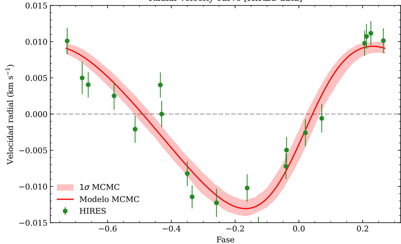
Radial Velocity curve [HIRES data]
