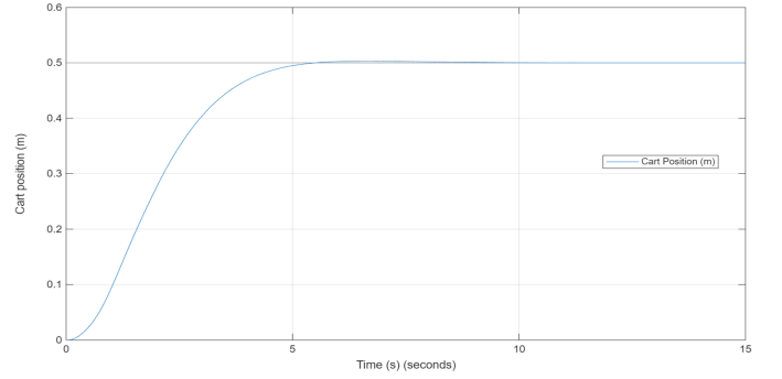
Fig. 4. Simulated cart position p(t) under LQR control for a 0.5 m step reference.
