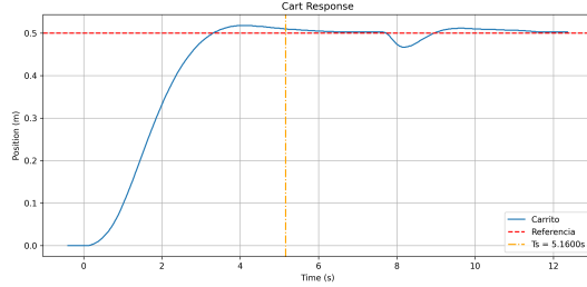
Fig. 2. Experimental step response of the cart position under Pole Placement control.
