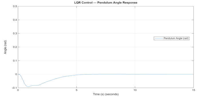
Fig. 5. Simulated pendulum angle \theta(t) under LQR control for a 0.5 m step reference.
