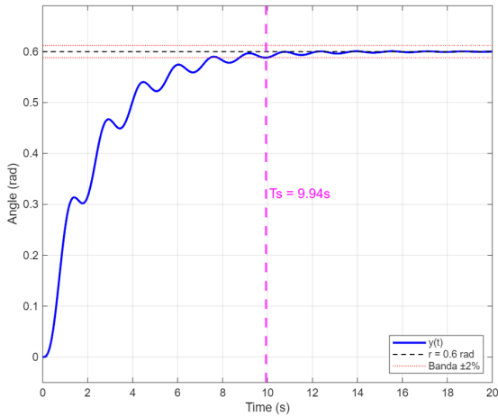
Fig. 4: Simulated step response of the ISF-LQR controller.
