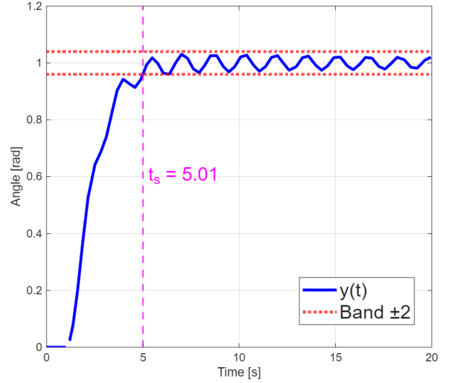
Fig. 1: Simulated step response of the PID controller.
