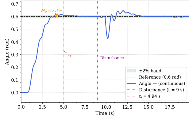
Fig. 5: Experimental step response of the ISF-LQR controller.
