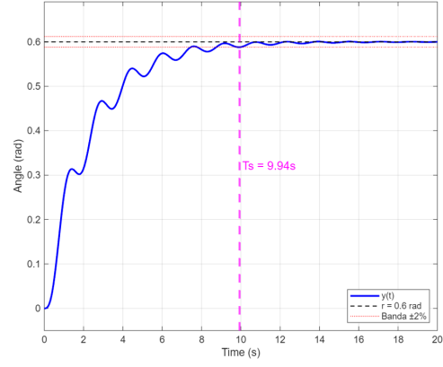
Fig. 4: Simulated step response of the ISF-LQR controller.
