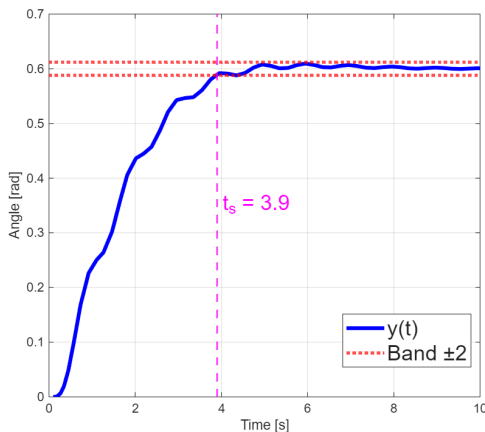
Fig. 6: Simulated step response of the I-PD controller.
