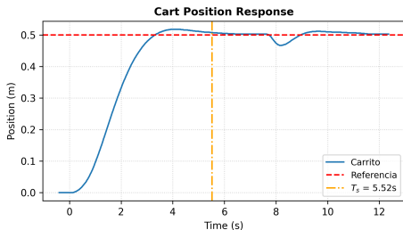
Fig. 2. Experimental step response of the cart position under Pole Placement control.
