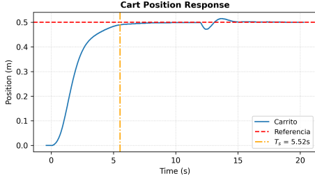
Fig. 6. Experimental cart position p(t) under LQR control for a 0.5 m step reference.
