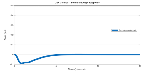
Fig. 5. Simulated pendulum angle \theta(t) under LQR control for a 0.5 m step reference.
