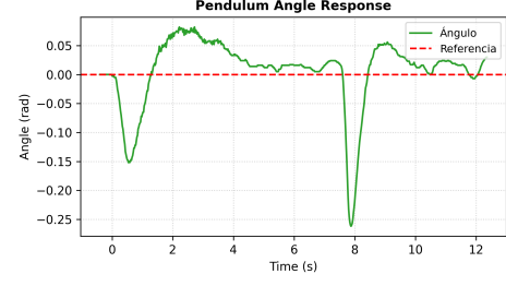
Fig. 3. Experimental pendulum deflection angle during the position step displacement under Pole Placement control.
