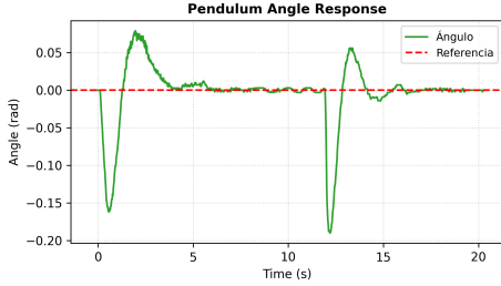
Fig. 7. Experimental pendulum angle \theta(t) under LQR control for a 0.5 m step reference.
