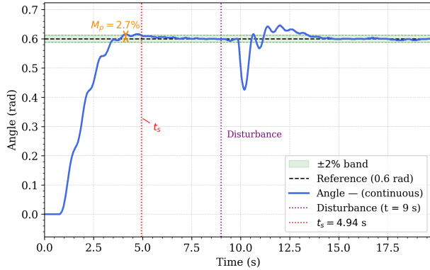
Fig. 5: Experimental step response of the ISF-LQR controller.
