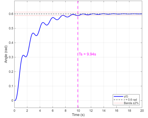
Fig. 4: Simulated step response of the ISF-LQR controller.
