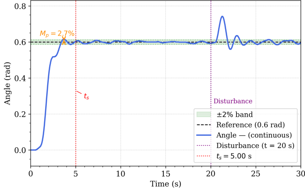
Fig. 2: Experimental step response of the PID controller.
