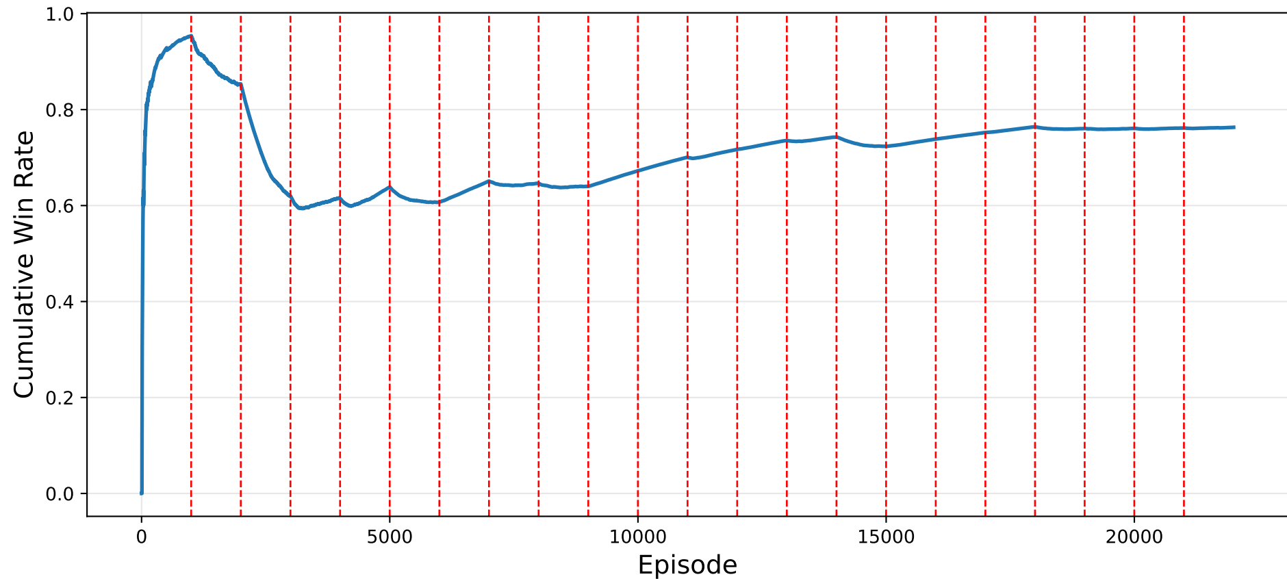
DQN Agent Training Performance
