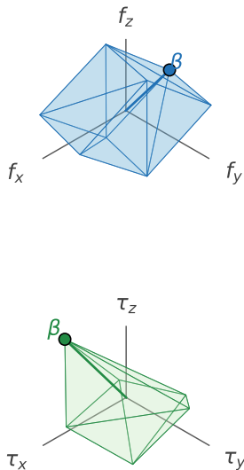
(b) grasp wrench space
