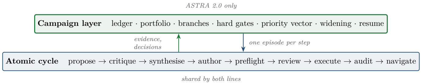
Figure 1: 2.0 does not replace the worker; it closes a loop around it. The upward arrow is the part 1.0 has no place to put.
