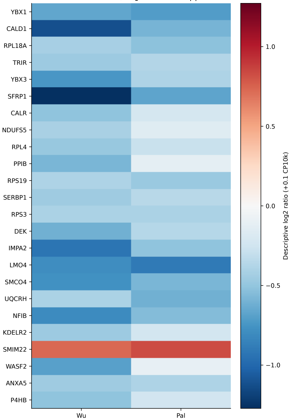
Up to 24 shared-direction genes P<0.05 in both; largest minimum |t|
